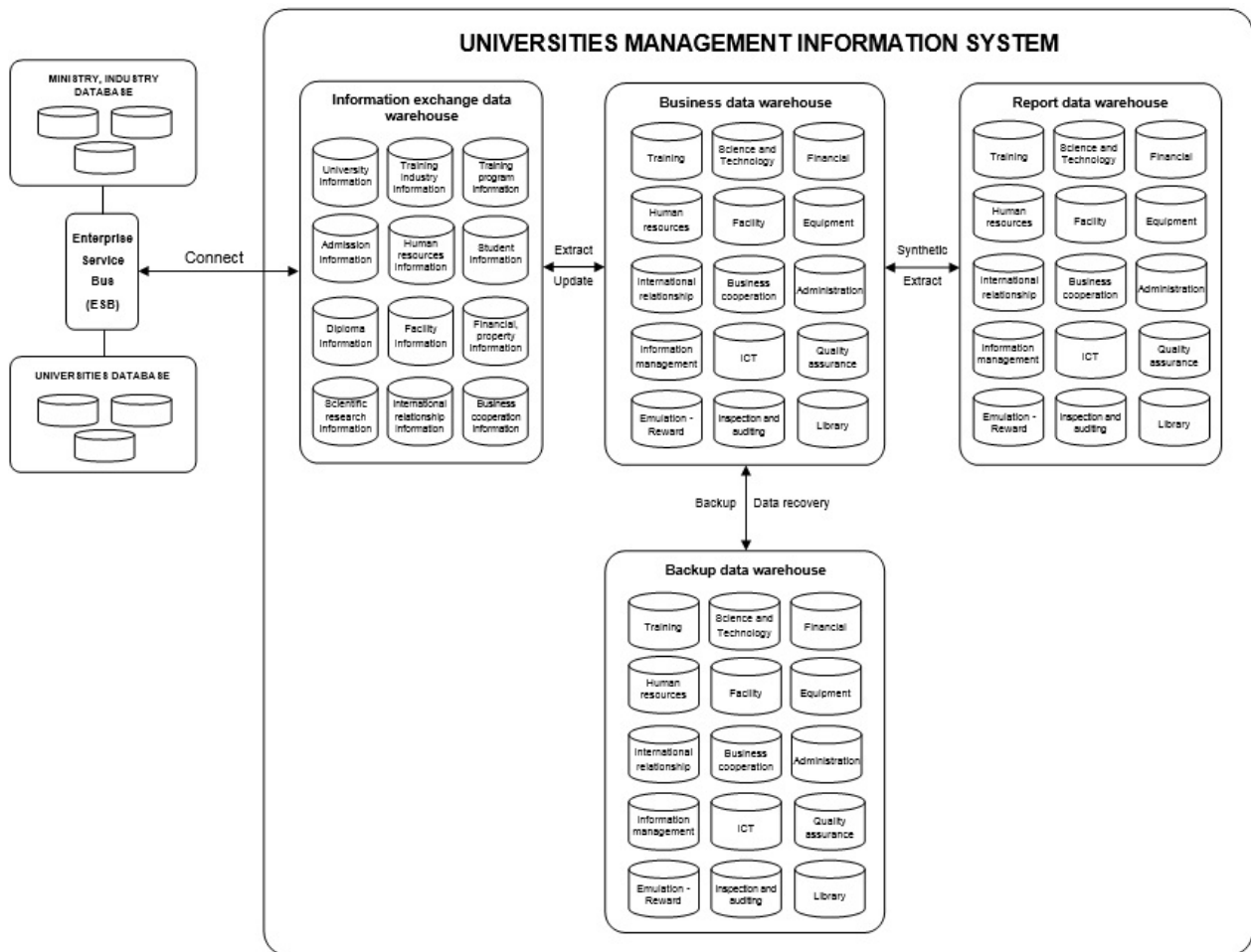
Fig. 4. Data Architecture
