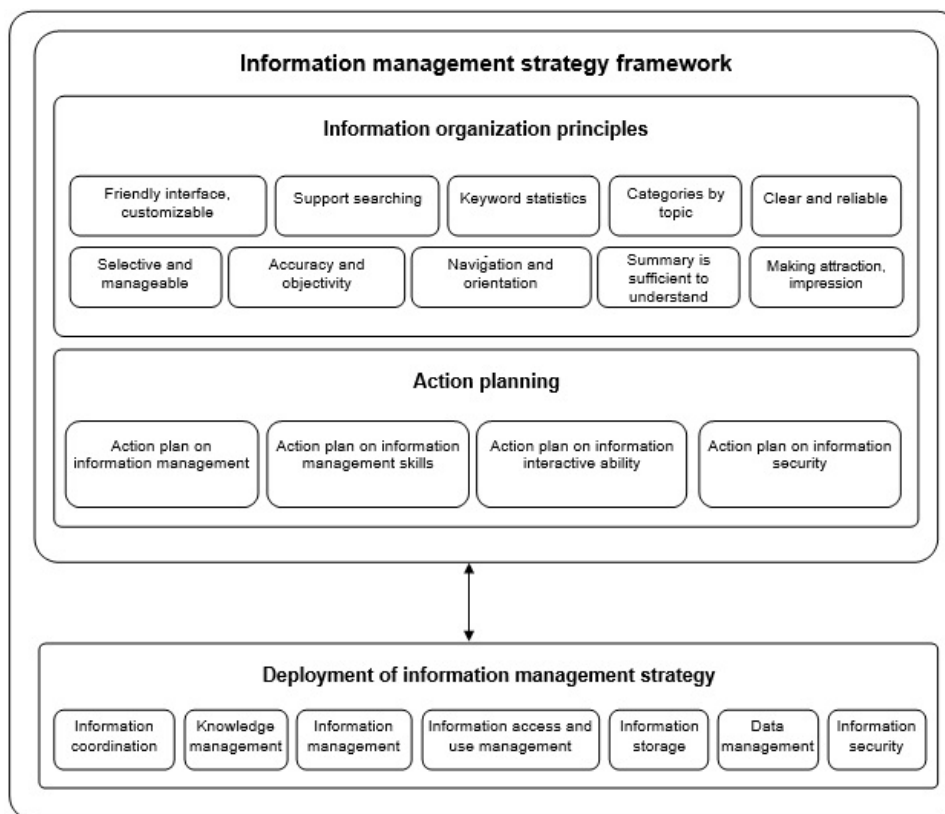
Fig. 7. Information Architecture
