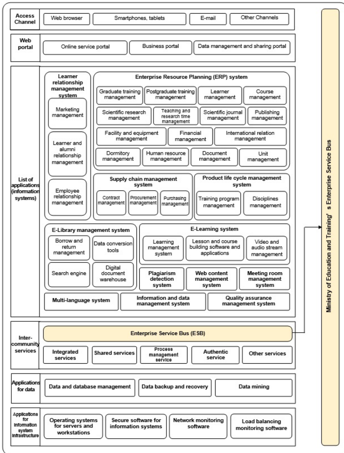
Fig. 5. Application Architecture
