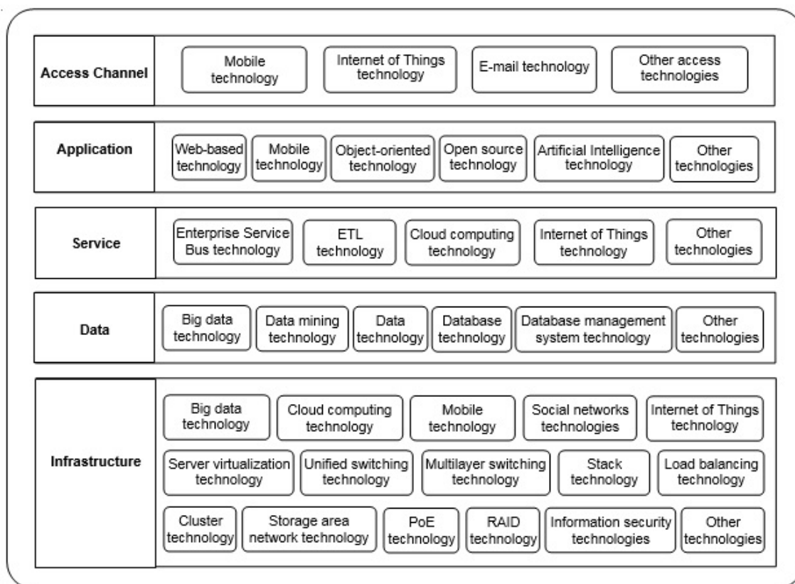
Fig. 6. Technology Architecture
