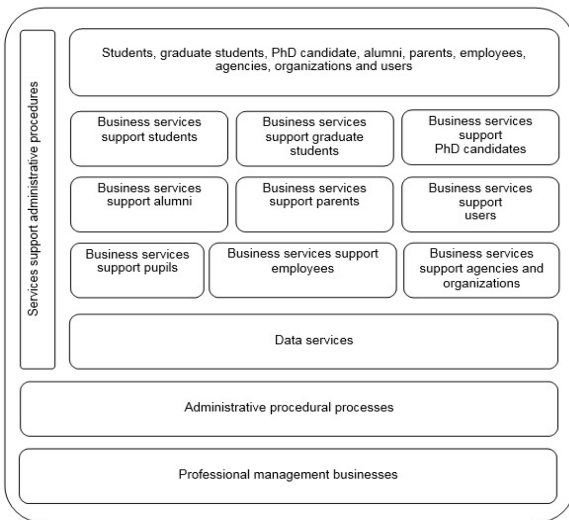
Fig. 3. Business Architecture
