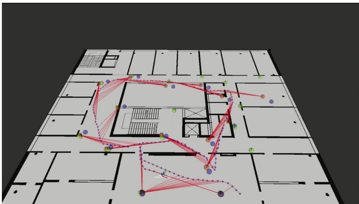
Рис. 4. Graph-based SLAM
