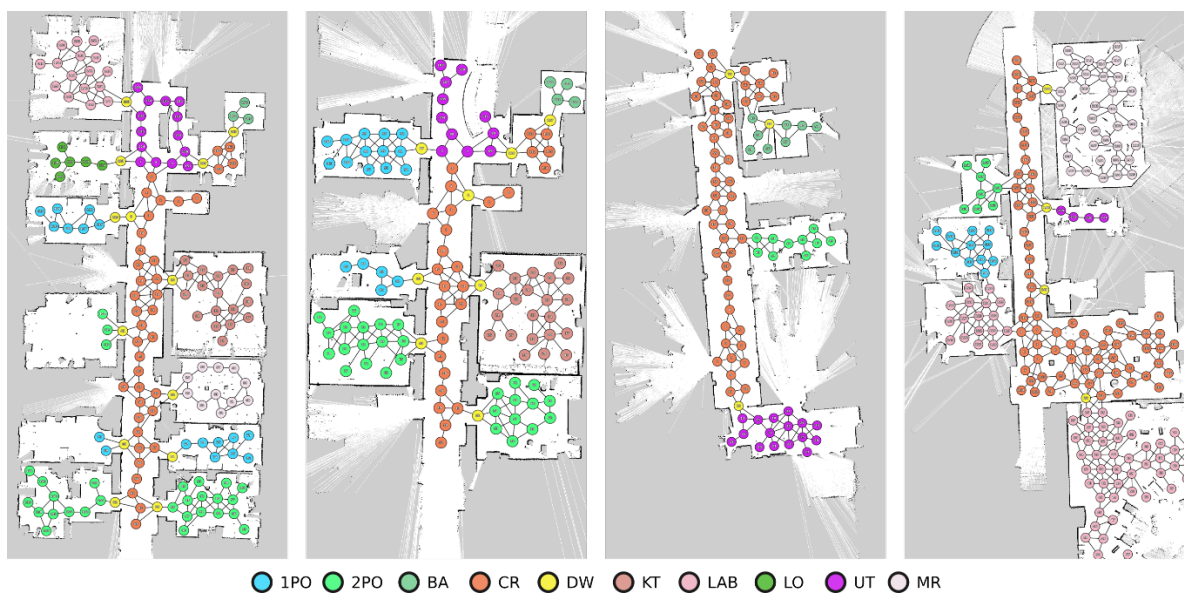
Рис. 6. Topological SLAM
