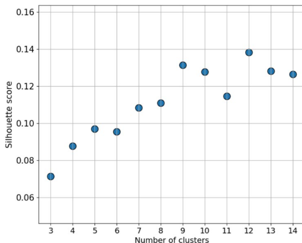
The silhouette coefficient method for determining number of clusters
