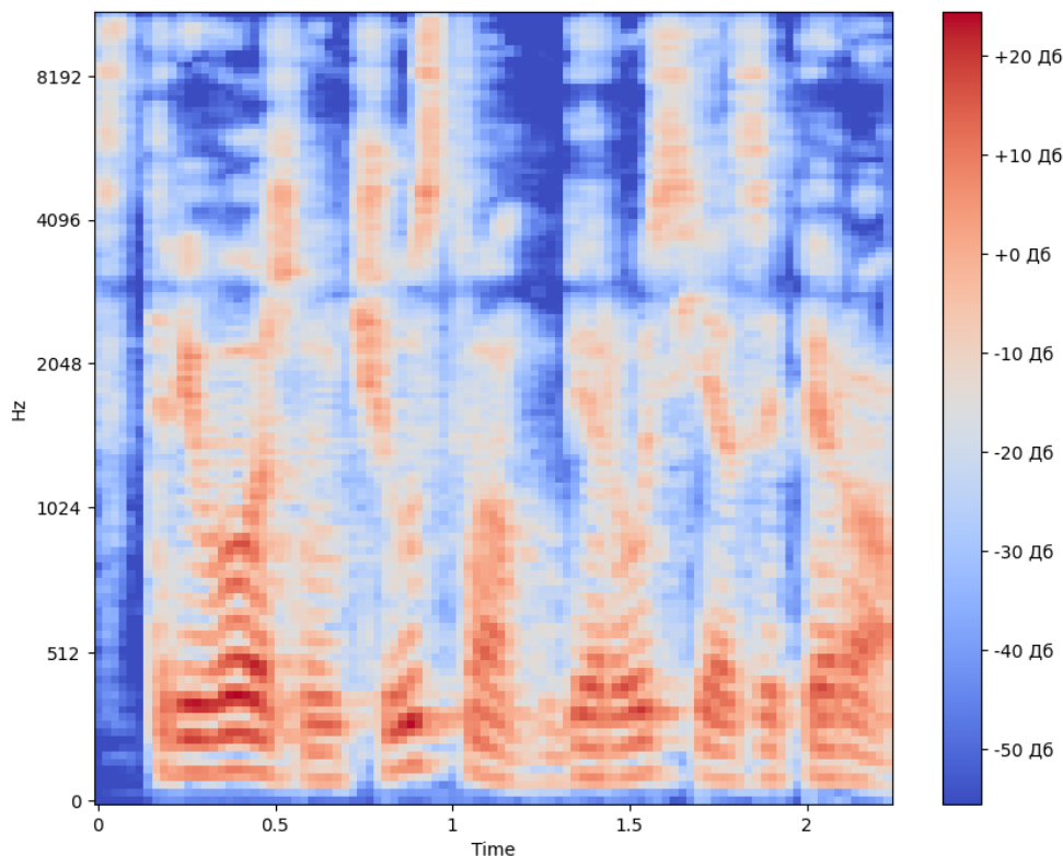
Pic. 4. Mel-spectrogram
