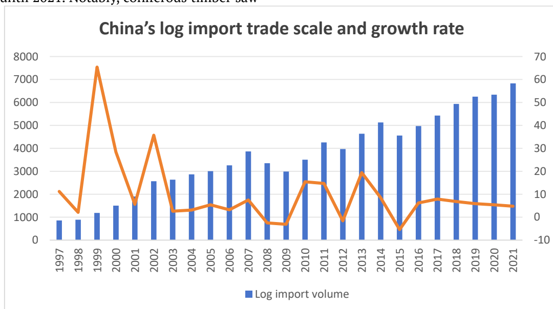
Fig. 1. The scale and growth rate of China's log import trade
