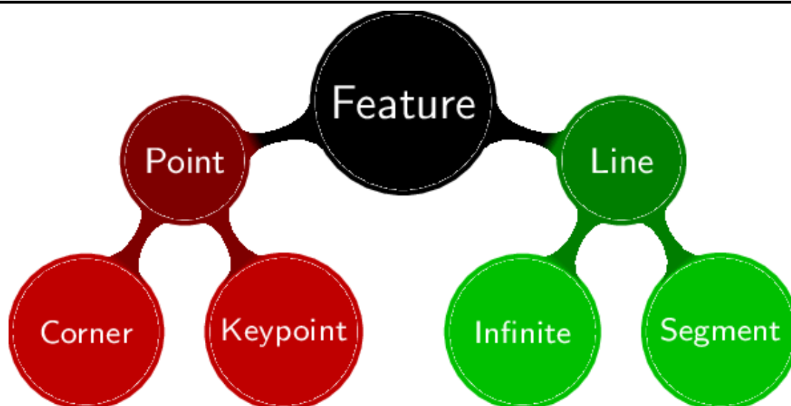
Рис. 3. Feature-based SLAM
