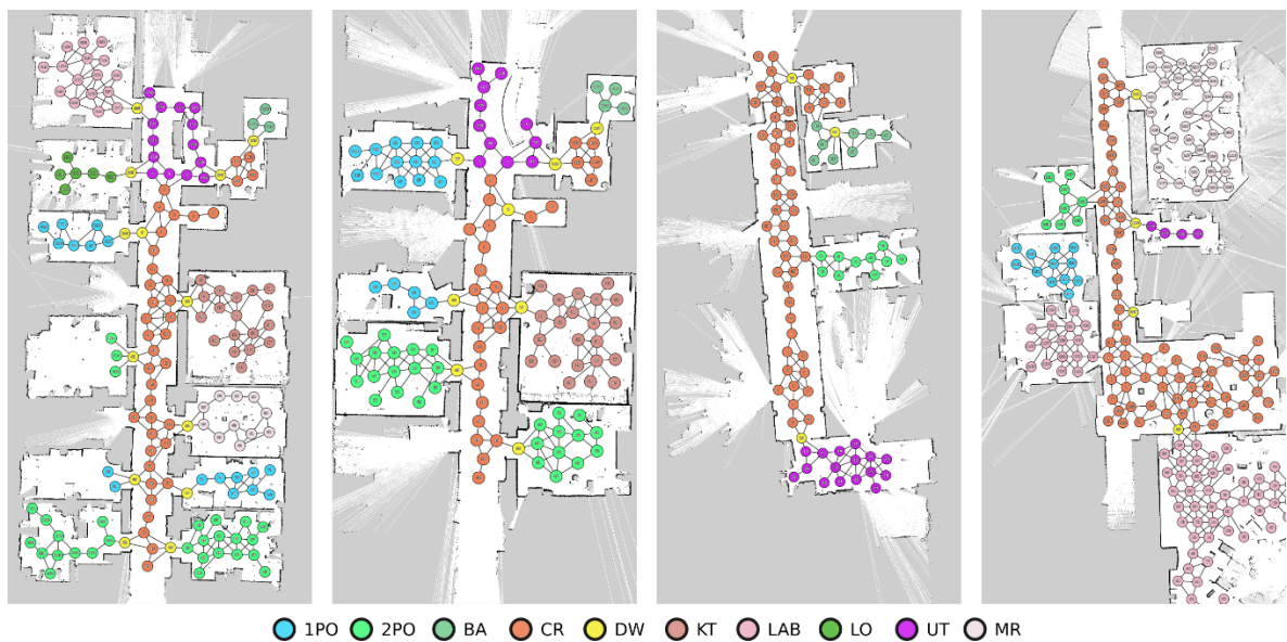
Рис. 6. Topological SLAM
