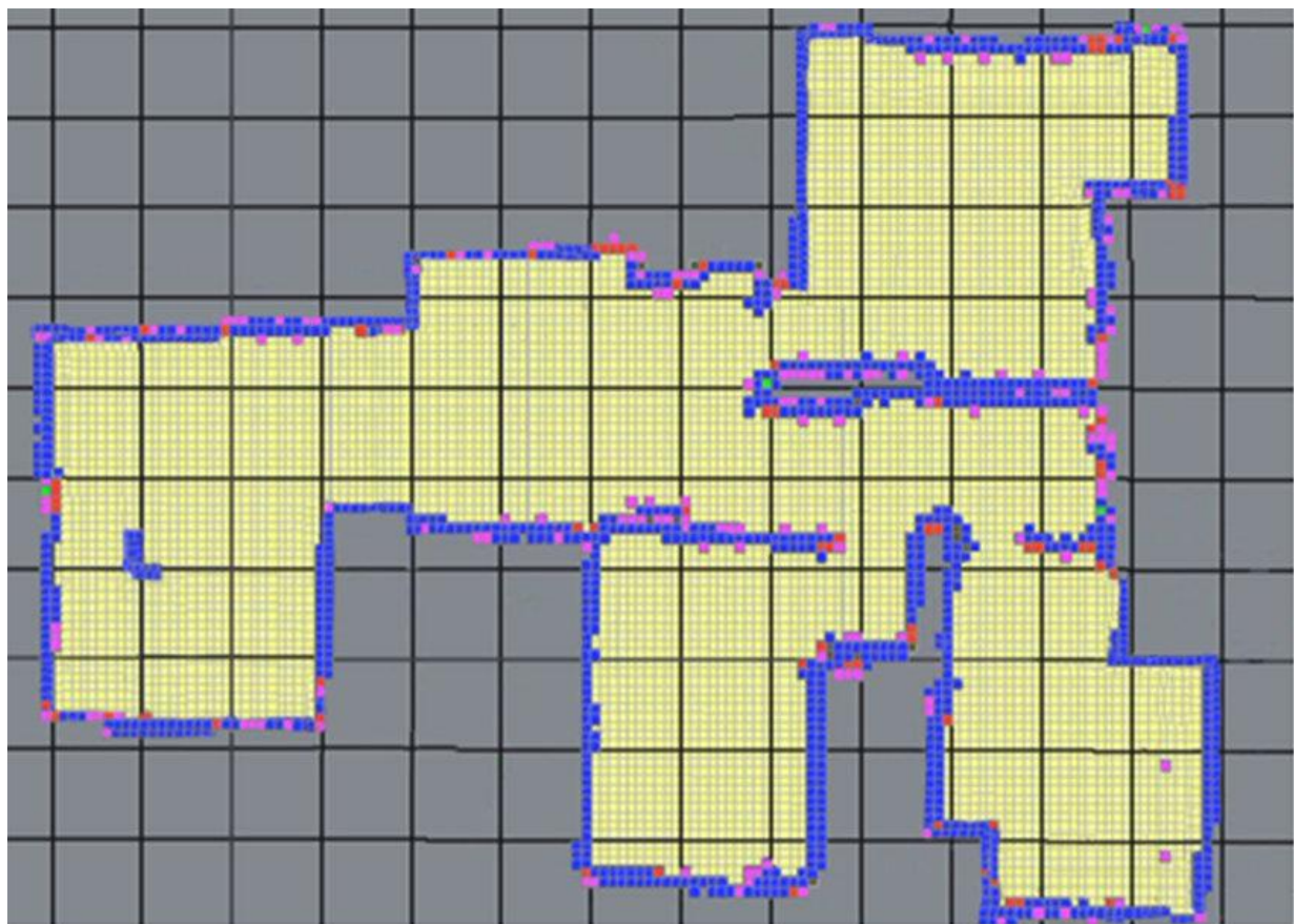
Рис. 5. Grid-based SLAM
