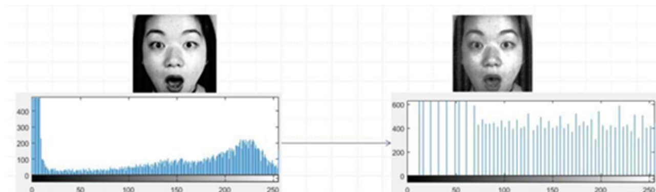
Fig. 9. Normalize an image using Histogram equalization
